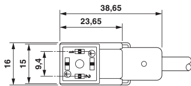
Valve connector, type CI
