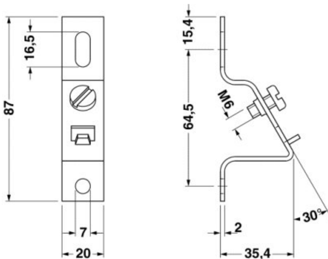
Dimensional drawing
