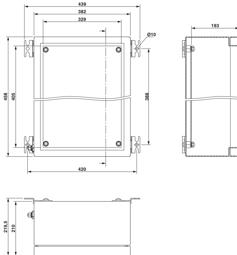
Dimensional drawing
